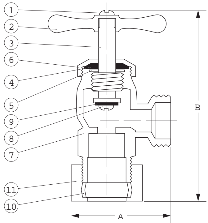
Pictured Model T-12 Cut-away
