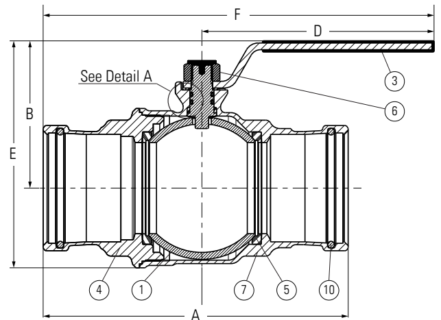
Pictured: P-200NL LegendPress® (2-1/2" to 4") Cut-away view
