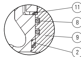
Pictured: P-200NL LegendPress® Stem area - Detail A
