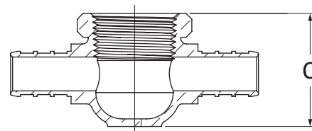
Pictured: PEX x FNPT Drop-ear tee Cut-away
