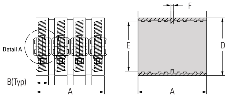
Pictured: 4" heavy-duty no hub, front view
