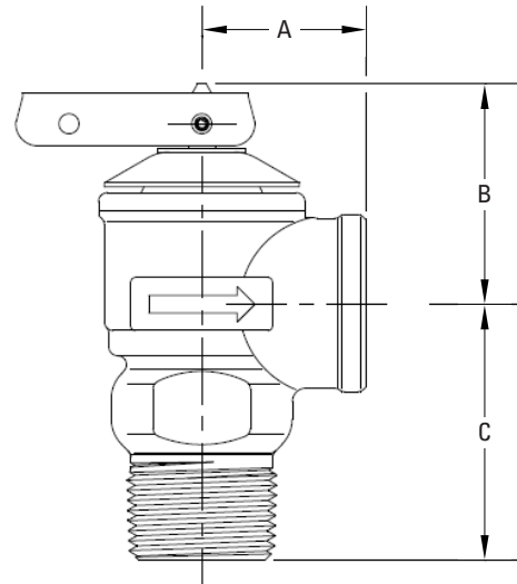
Pictured: Pressure Relief Valve Dimensional Reference
