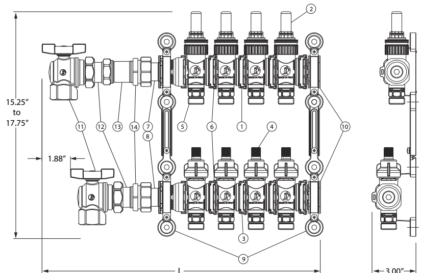
Pictured: M-8100A 4-Circuit manifold
