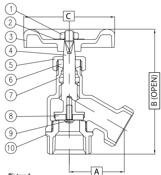
Pictured: T-543NL Bent-nose garden valve Cutaway view
