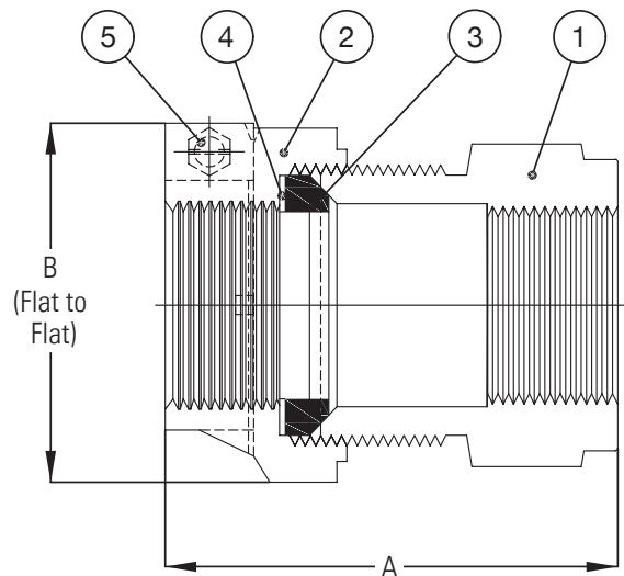
Pictured: T-4305NL Cut-away
