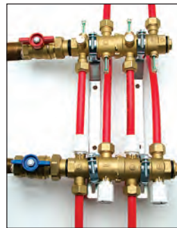
M-8000 Modular™ Manifold circuit sections rotate allowing tube to be routed from above or below the manifold offering the ultimate in job site flexibility
